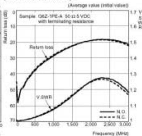
High-frequency Characteristics at 50 Ω (Return Loss, V.SWR)
