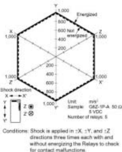
Shock Malfunction
