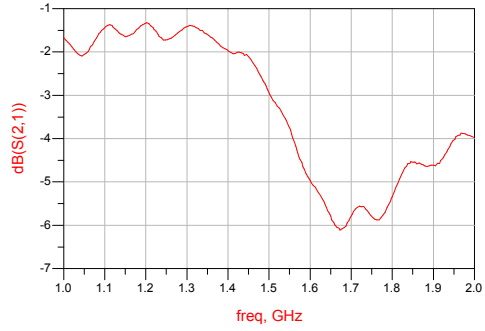
IN-OUT-12V Isolation
