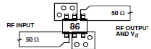
Figure 13. RF Layout.
