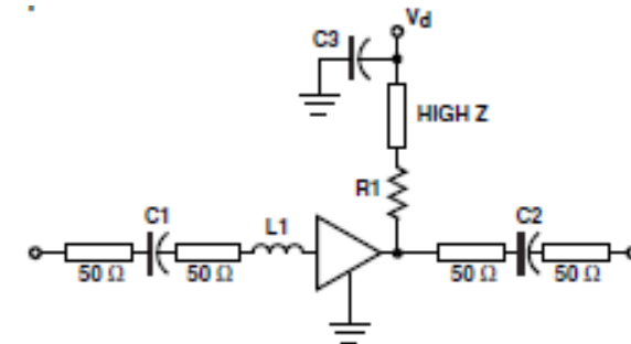
Figure 14. Typical Amplifier Circuit.
