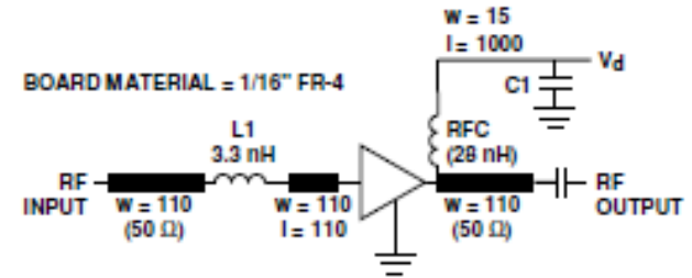
Figure 10. Test Circuit for 2 GHz.
