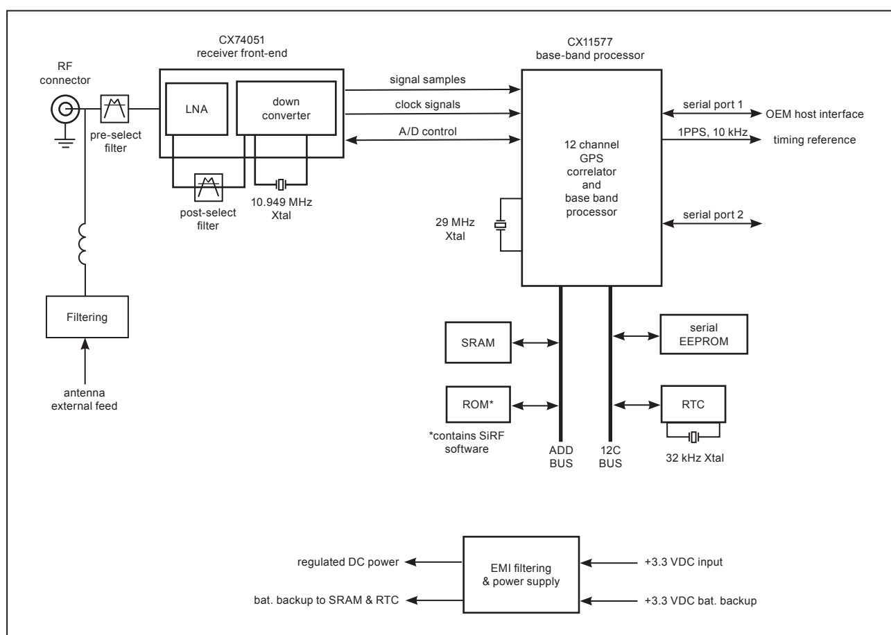
Figure 1-3. Jupiter Pico T block diagram
