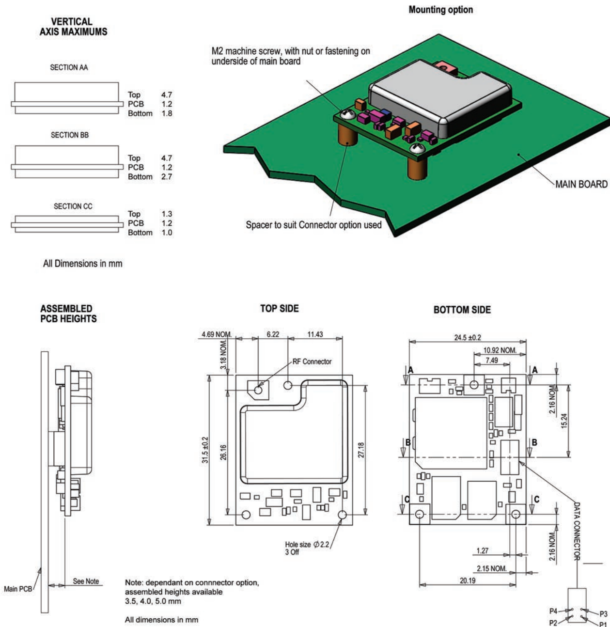
Figure 3-4 Jupiter Pico GPS receiver board (dimensions mm) (vertical sections do not include protrusions due to I/O connector dimensions)
